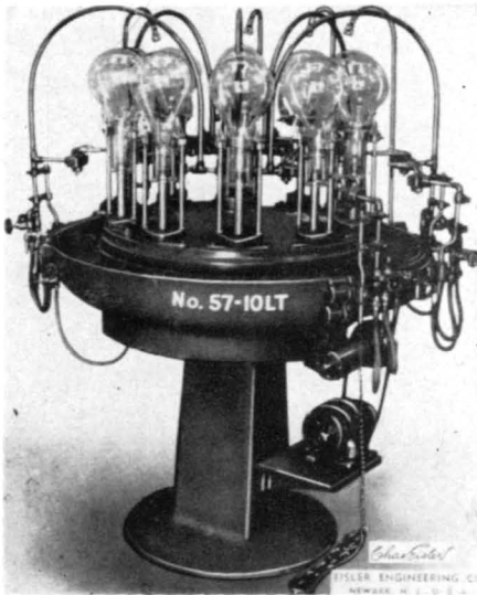
The Eisler 10-head automatic sealing machine.
